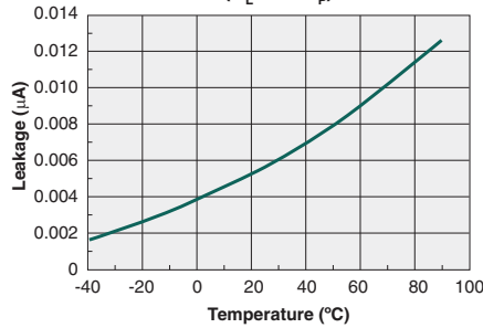
Typical Leakage vs. Temperature Measured Across Pins 1&2 ( V_L=800\text{V}_p )
